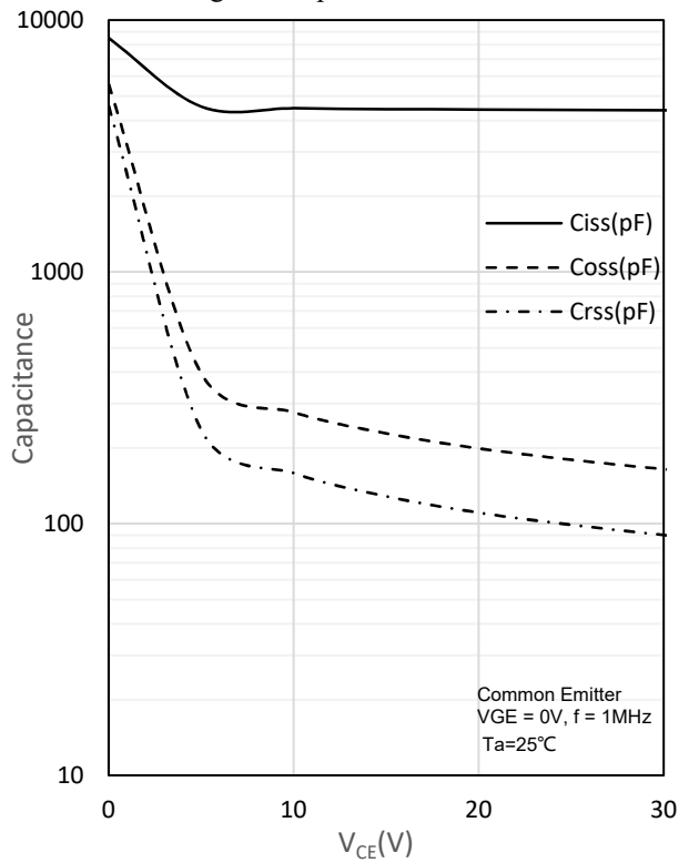
Fig. 12 Capacitance characteristics
