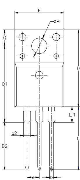
TO-220FJ-3L
